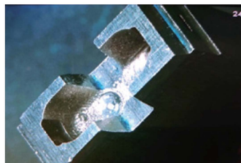
Mold Inspection
